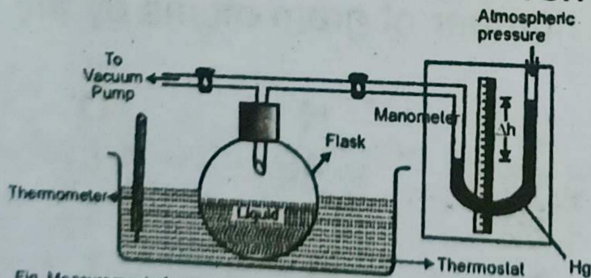
Fig. Measurement of vapour pressure of a liquid by manometric method.
