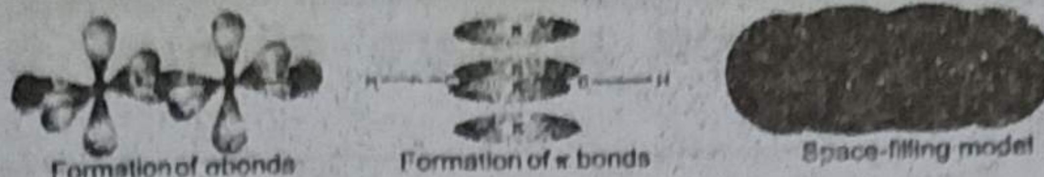
Fig. Formation of ethyne.
